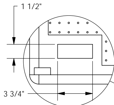
DETAIL VIEW
