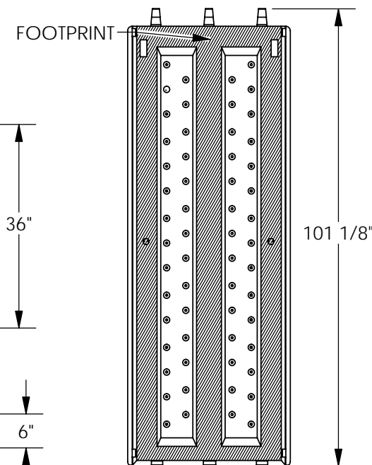
BOTTOM VIEW
